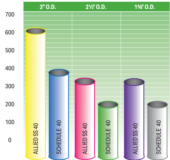
Test results are based on 6 foot cantilevered beam test and 10 foot free-supported beam test.
